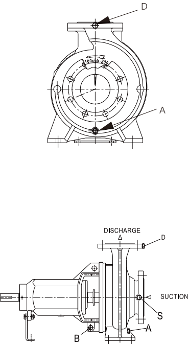
Service Connections
